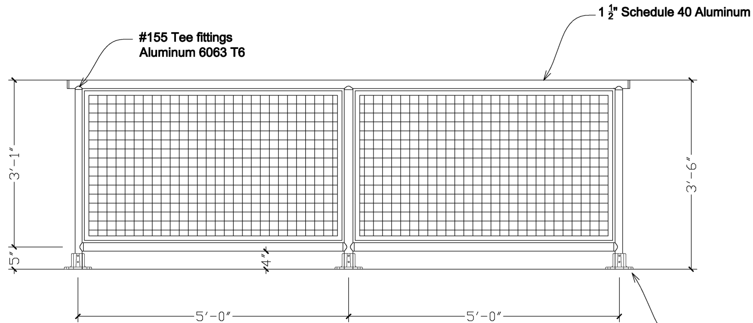
Base Mount Flange * See flange chart
